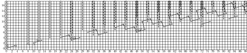
The Adams spectral sequence \text{Ext}_{A_3^{tmf}}(\mathbb{F}_3, \mathbb{F}_3) \Rightarrow \pi_*(tmf)_3^\wedge .
